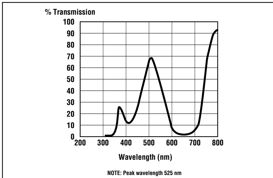
Figure 1. Percent transmission of light wavelengths through the FLTG green filter
