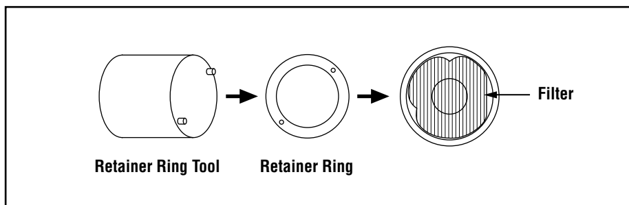
Figure 2. Installing the FLTG green filter on the camera
