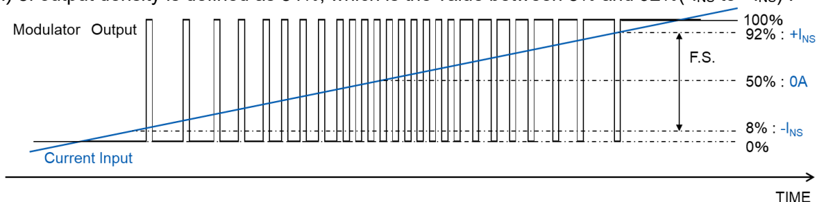
Figure 3. Typical output characteristics of CQ-360x
