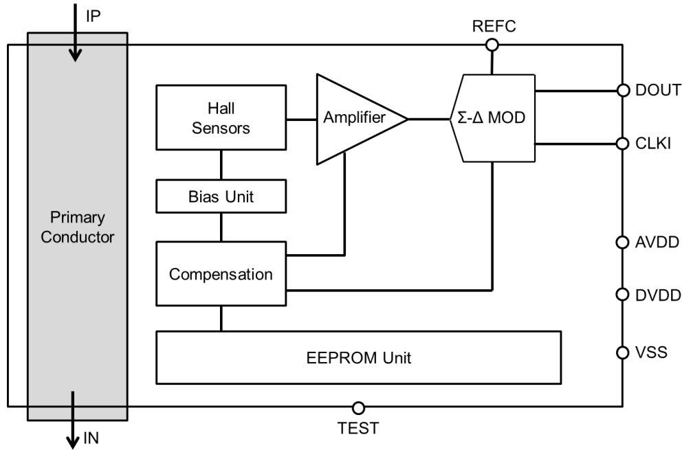
Figure 1. Block diagram of CQ-360x
