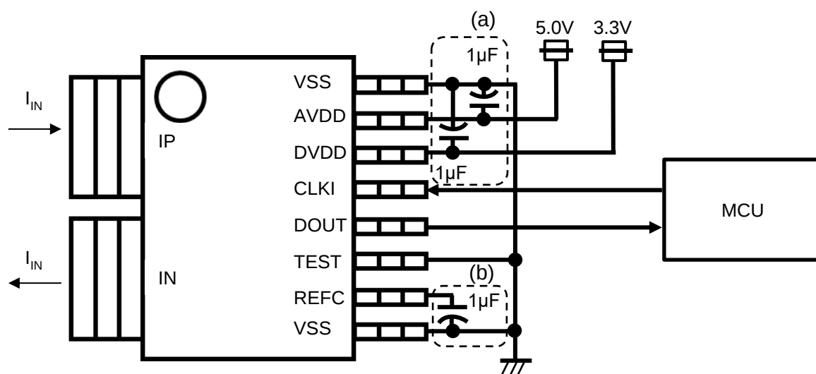
Figure 7. Recommend External Circuit of CQ-360x
