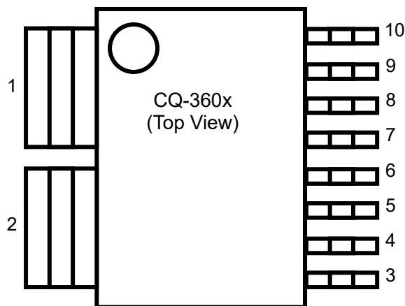
Figure 2. Pin configurations of CQ-360x
