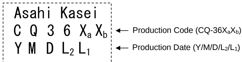
Figure 11. Markings of CQ-360x
