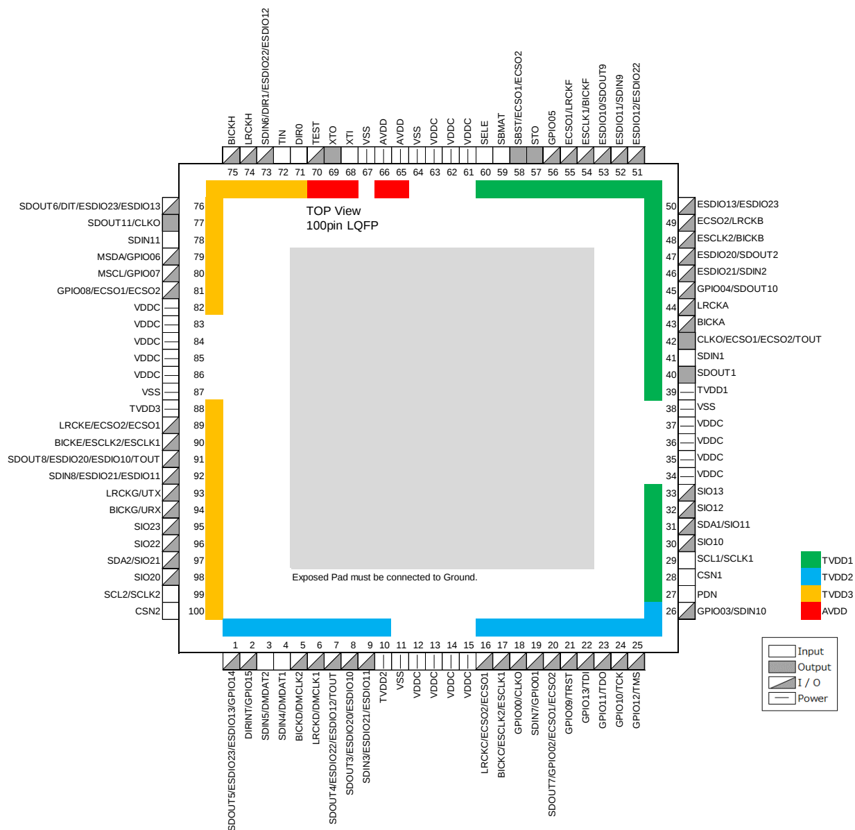
Figure 3. Pin Configurations
