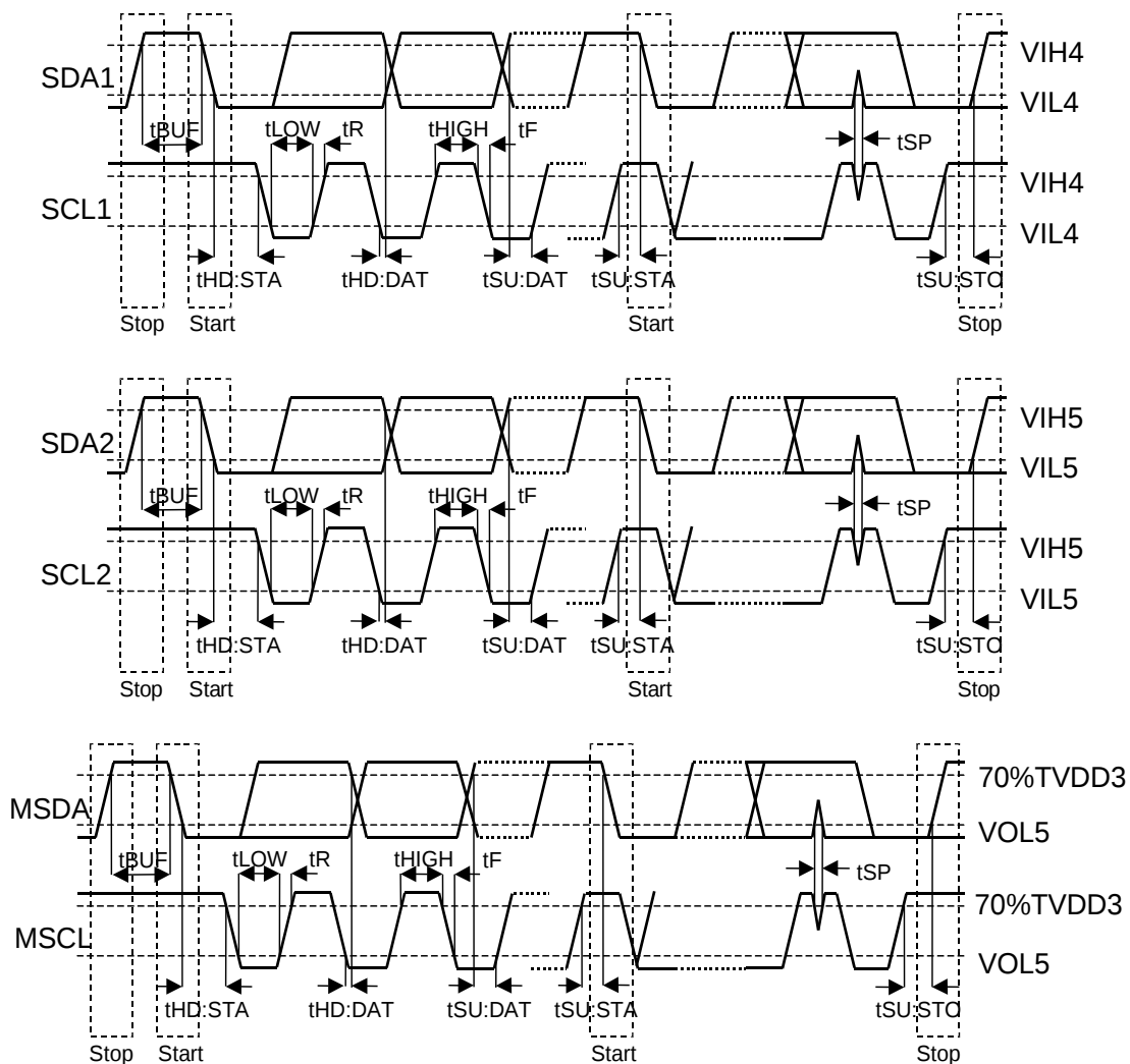
Figure 15. I²C BUS Interface Timing
