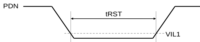
Figure 5. Reset Timing
