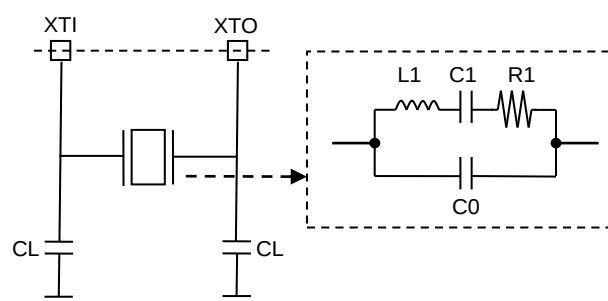
Figure 19. Electric Equivalent Circuit of Crystal Oscillator
