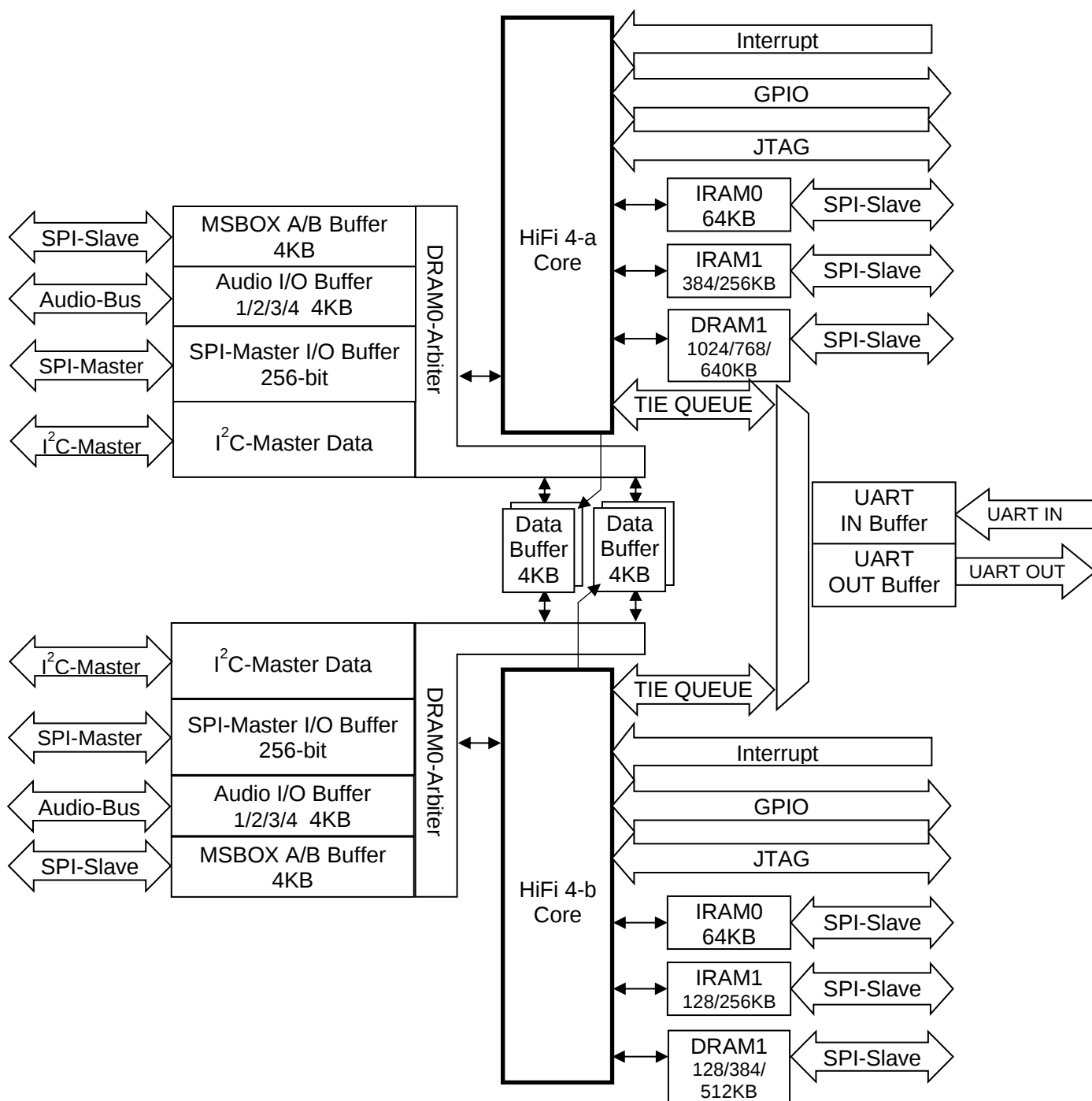
Figure 2. DSP1(HiFi 4-a), DSP2(HiFi 4-b) Block Diagram
