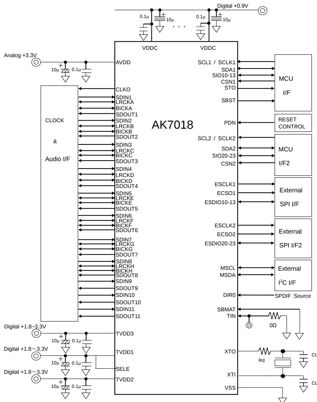
Figure 18. Connection Example
