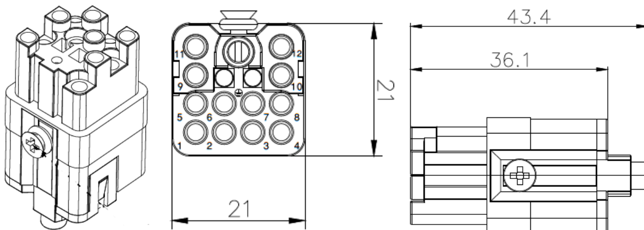
Technical Drawing and Polar Pattern female FCC
