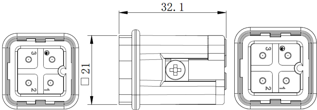
Technical Drawing and Polar Pattern male MCC
