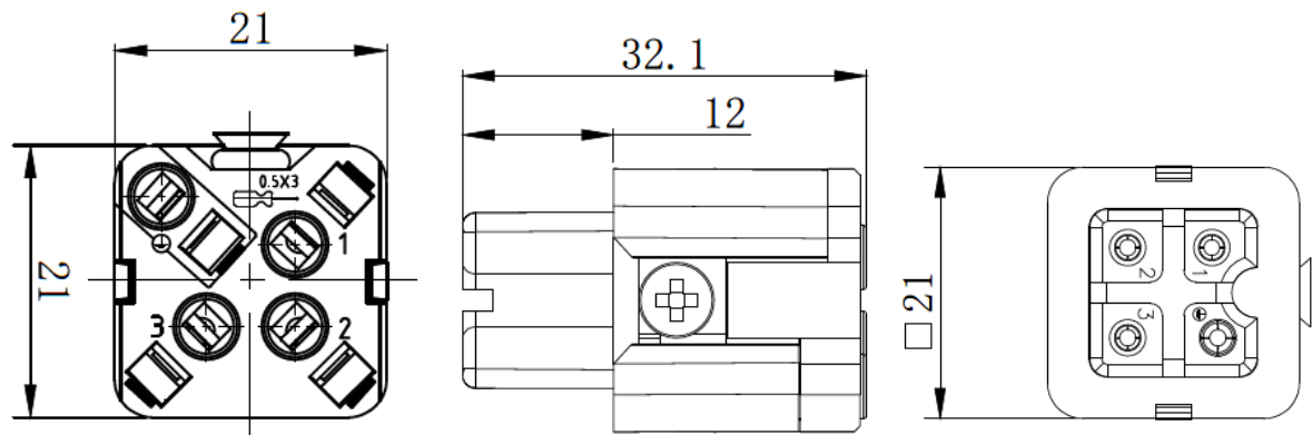
Technical Drawing and Polar Pattern female FCC
