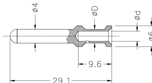
Drawing male contact
