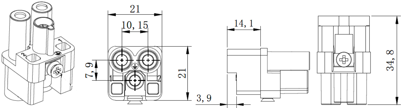
Technical Drawing and Polar Pattern male MCC
