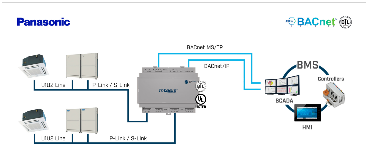
Figure 3. Integration of Panasonic units into BACnet systems
