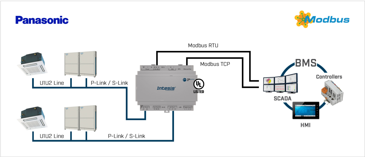
Figure 1. Integration of Panasonic units into Modbus systems
