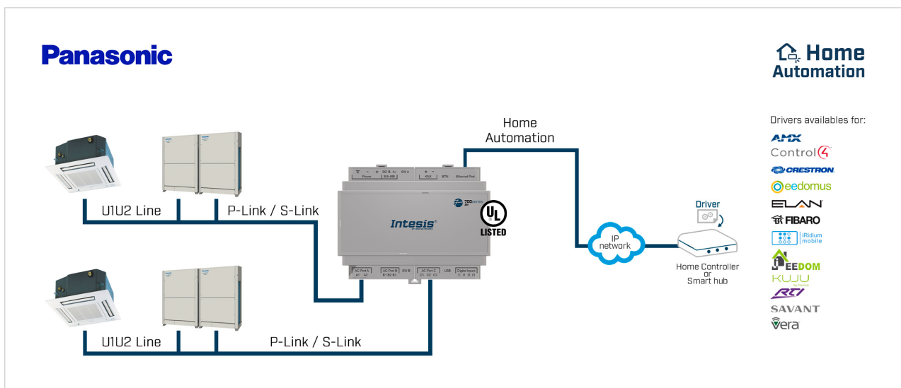
Figure 4. Integration of Panasonic units into Home Automation systems
