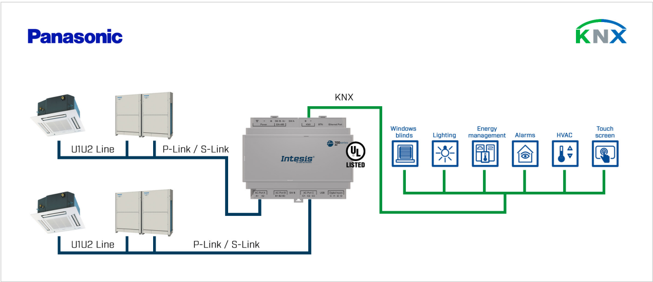
Figure 2. Integration of Panasonic units into KNX TP systems
