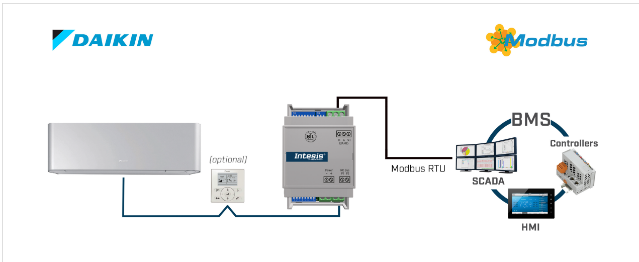
Figure 2. Integration of Daikin AC units into a Modbus RTU installation using the Intesis IN485DAI001R000 gateway.
