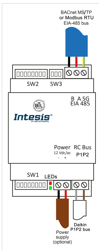
Figure 3. Wiring diagram
