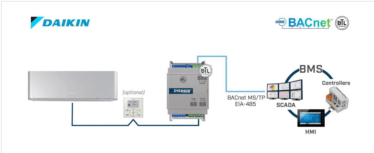
Figure 1. Integration of Daikin AC units into a BACnet MS/TP installation using the Intesis IN485DAI001R000 gateway.
