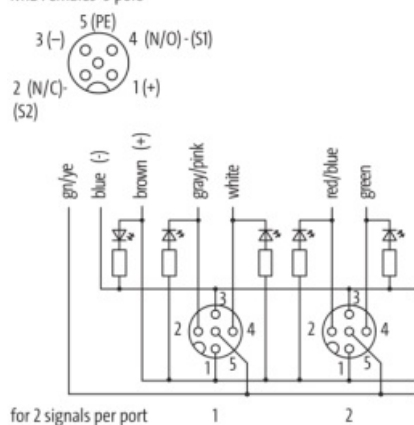
M12-Females 5-pole
