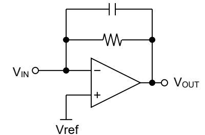
Transimpedance amplifier
