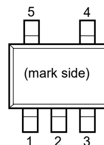
RP173N (SOT-23-5) Pin Configuration
