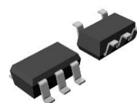
SOT-23-5 2.9 x 2.8 x 1.1 (mm)
