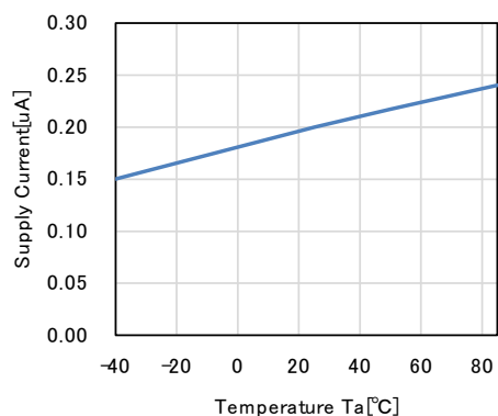
RP118x121x, V_{IN} = 2.2 V
