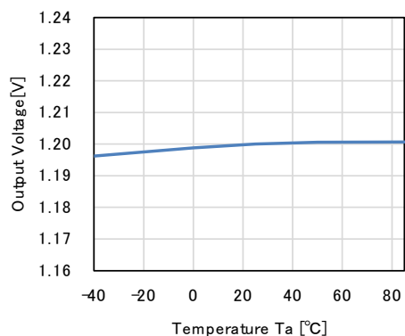
RP118x281x, V_{IN} = 3.8 V, I_{OUT} = 1 mA
