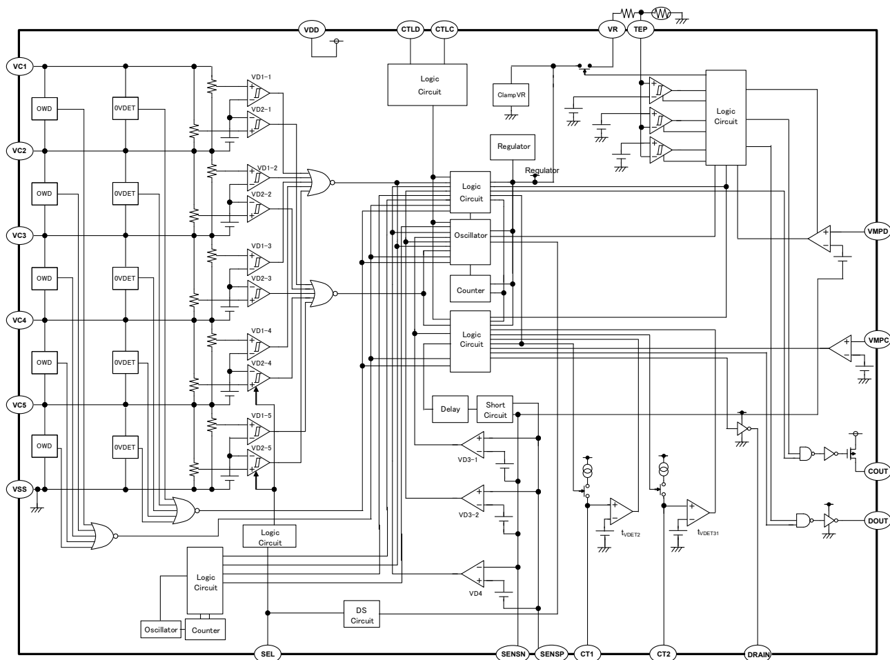
R5651T Block Diagram
