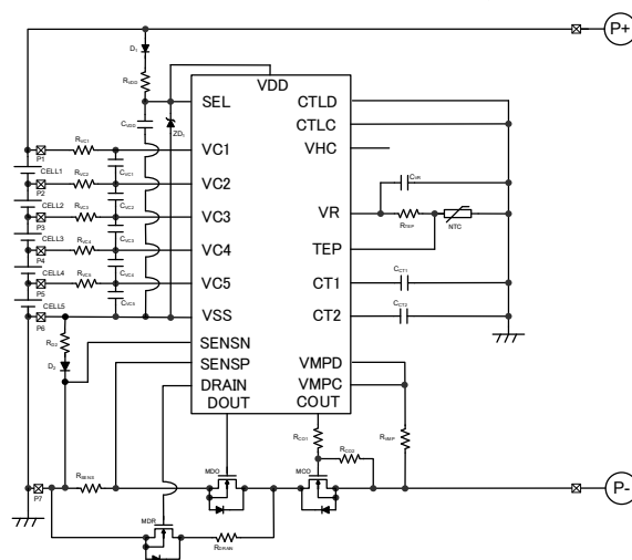
5-cell Protection Circuit (CMOS output type)
