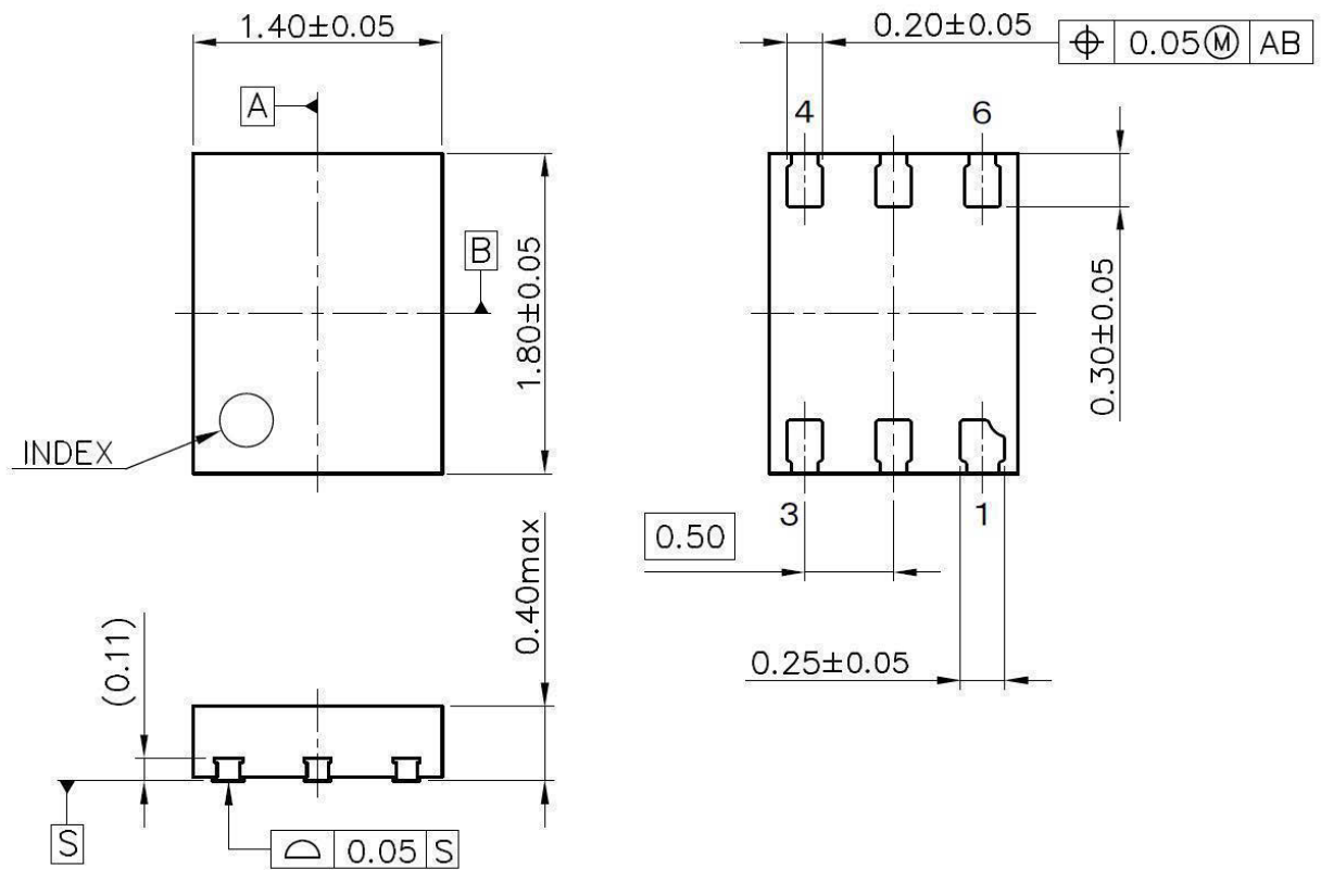
DFN1814-6B Package Dimensions (Unit: mm)
