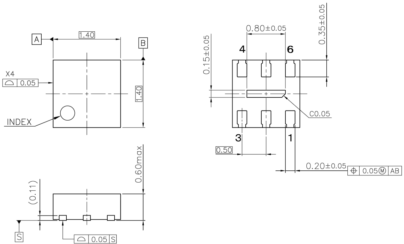
DFN1414-6B Package Dimensions (Unit: mm)
