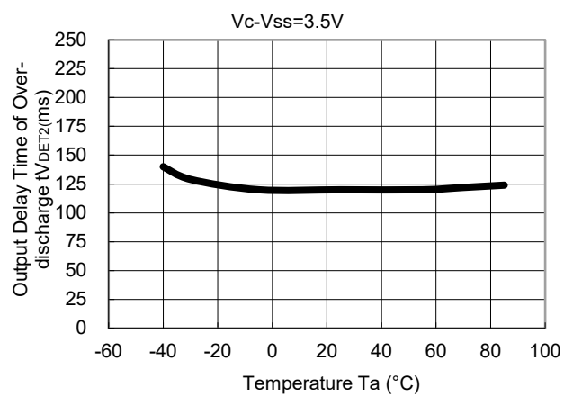
12) Output Delay Time for Over-discharge vs. Temperature R5460x201AC
