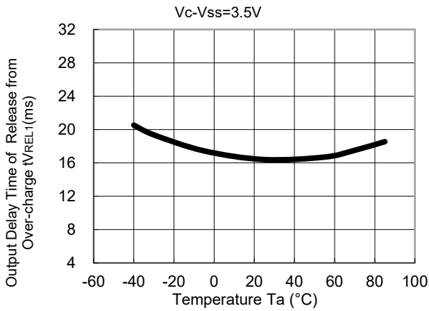
7) Output Delay of Release from Over-charge vs. Temperature R5460x201AC
