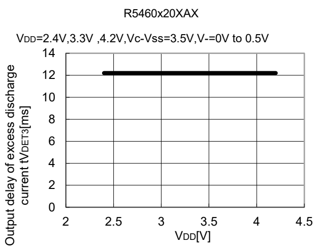
5) Output Delay for Excess Discharge Current vs. V DD
