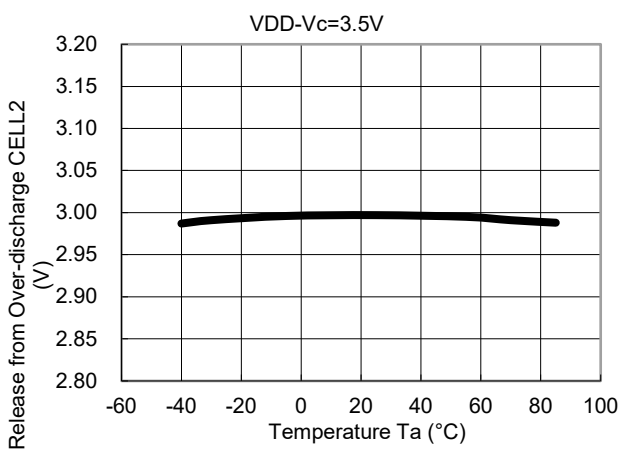
11) Release Voltage from Over-discharge (Cell2) vs. Temperature R5460x202AA
