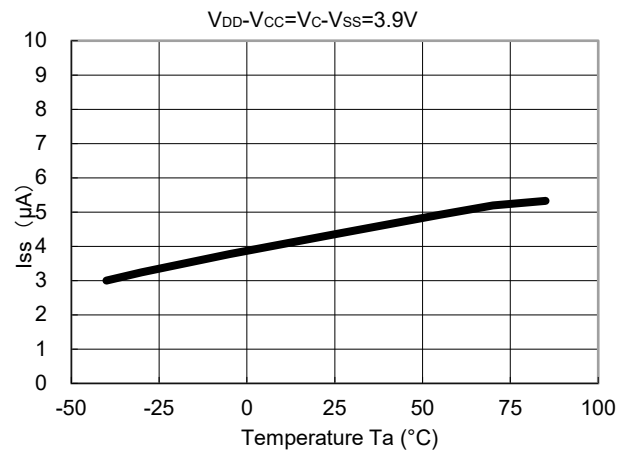
28) Supply Current vs. Temperature R5460x201AC
