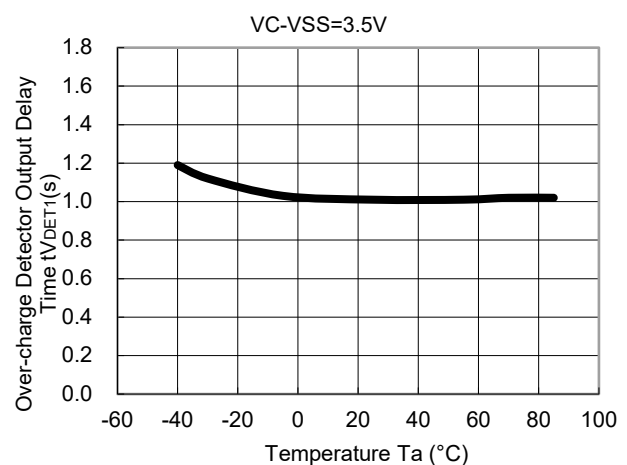
6) Output Delay of Over-charge Detector vs. Temperature R5460x201AC
