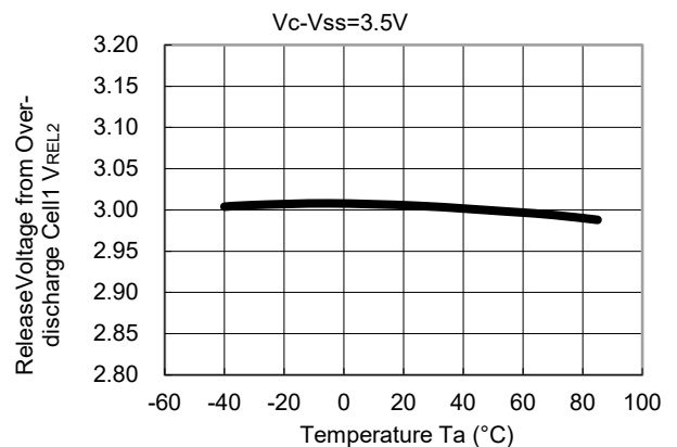
10) Release Voltage from Over-discharge (Cell1) vs. Temperature R5460x202AA
