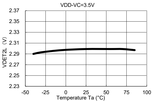
9) Over-discharge Detector Threshold (Cell2) vs. Temperature R5460x201AC
