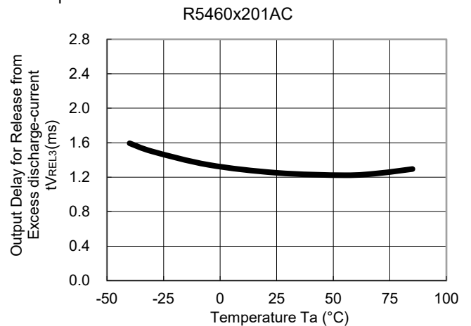
16) Output Delay for Release from Excess discharge-current vs. Temperature R5460x201AC
