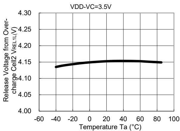
5) Release Voltage from Over-charge (Cell2) vs. Temperature R5460x201AC
