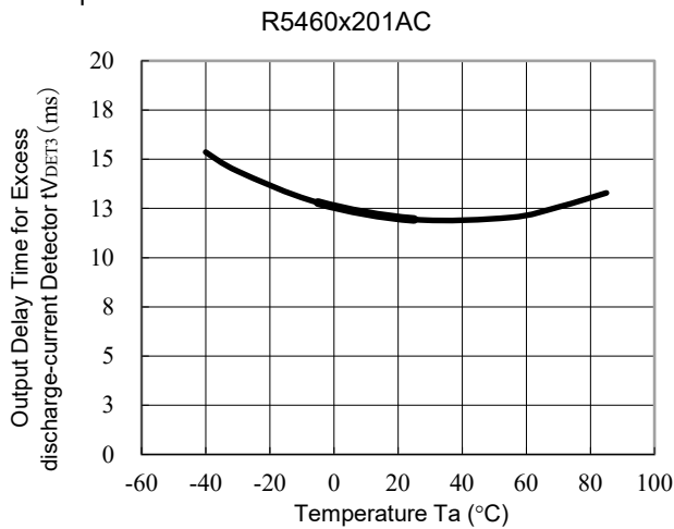
15) Output Delay Time for Excess discharge-current Detector vs. Temperature R5460x201AC
