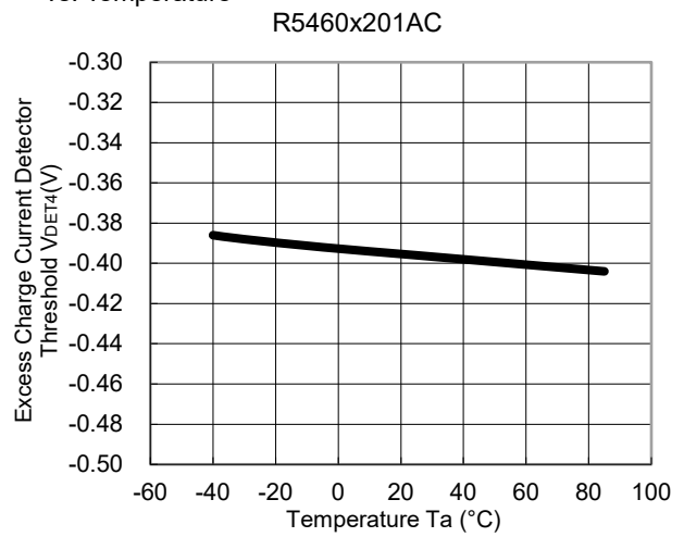
20) Excess-charge current Detector Threshold vs. Temperature
