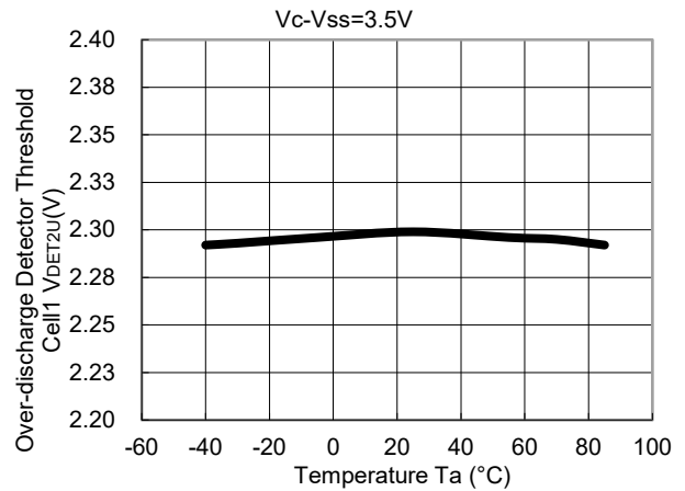
8) Over-discharge Detector Threshold (Cell1) vs. Temperature R5460x201AC
