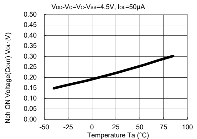
24) Nch ON Voltage of COUT vs. Temperature
