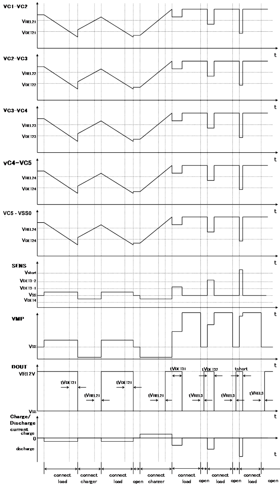
Overdischarge / Discharge Overcurrent / Short-circuit Operation Timing Chart
