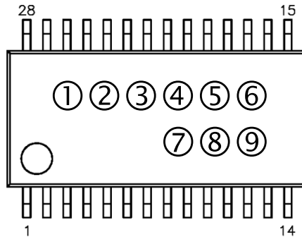
R5436T (TSSOP-28) Part Markings
