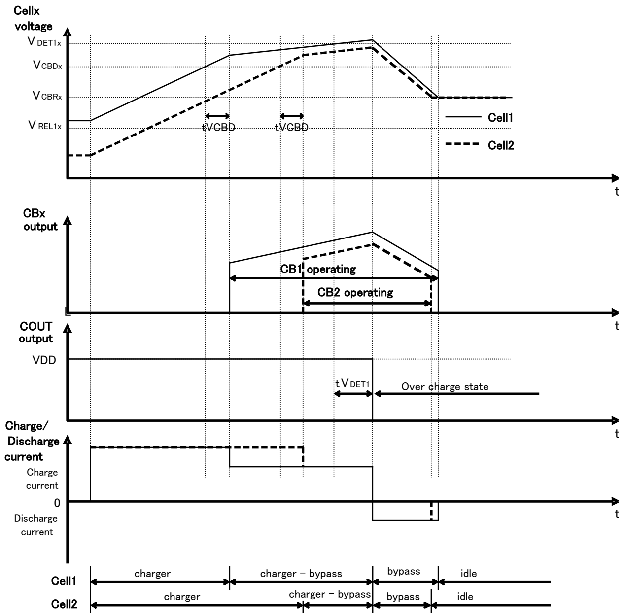
CELL1/2 Balancing Timing Chart
