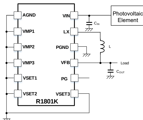
Test Circuit for Typical Characteristics 5)
