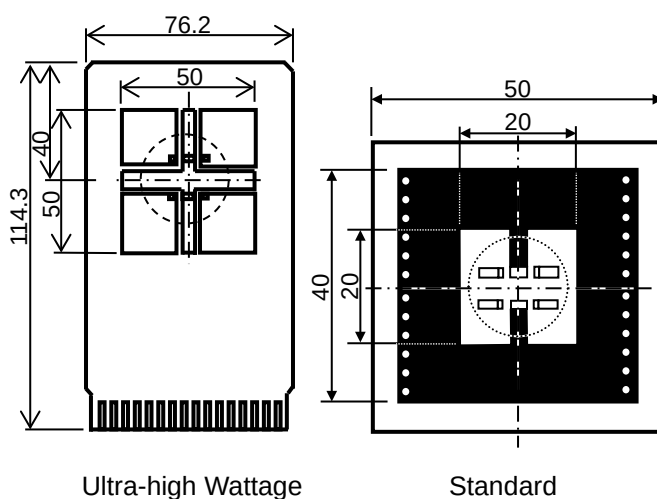
○ IC Mount Area (mm)
