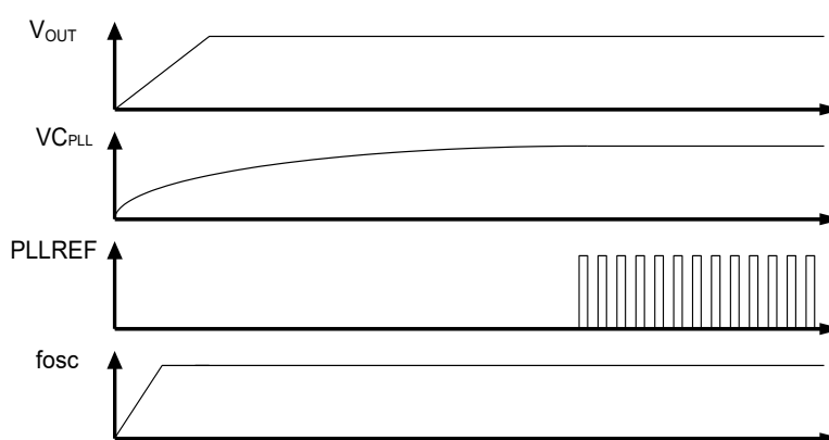
R1270S001A/B PLL Filter Start-up Sequence Phase Compensation Filter Charging Time < Synchronous Start Time with External Clock
