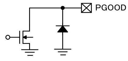
< PGOOD Pin >
