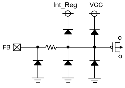
< FB Pin >
