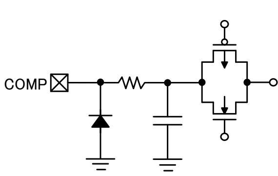
< COMP Pin >
