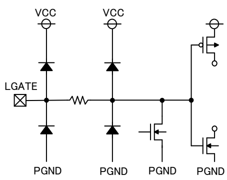
< LGATE Pin >
