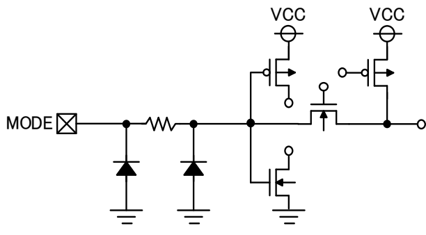
< MODE Pin >
