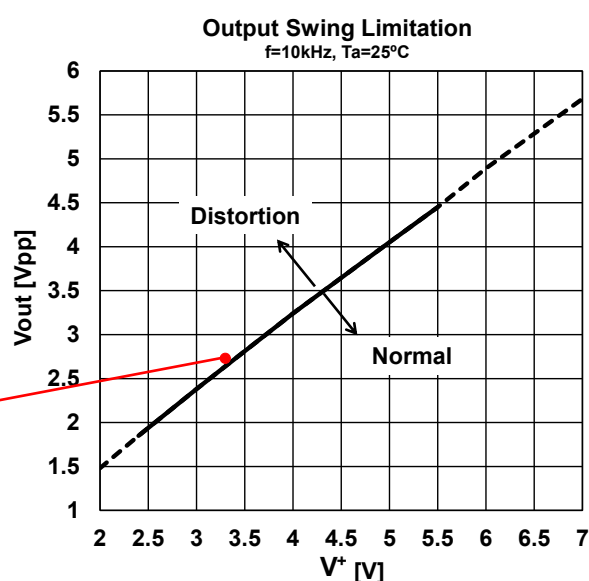
Figure5-2. Output voltage limit
