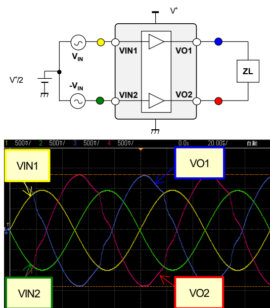
Figure5-1. Waveform at large amplitude ( Z_L : Resolver model)
