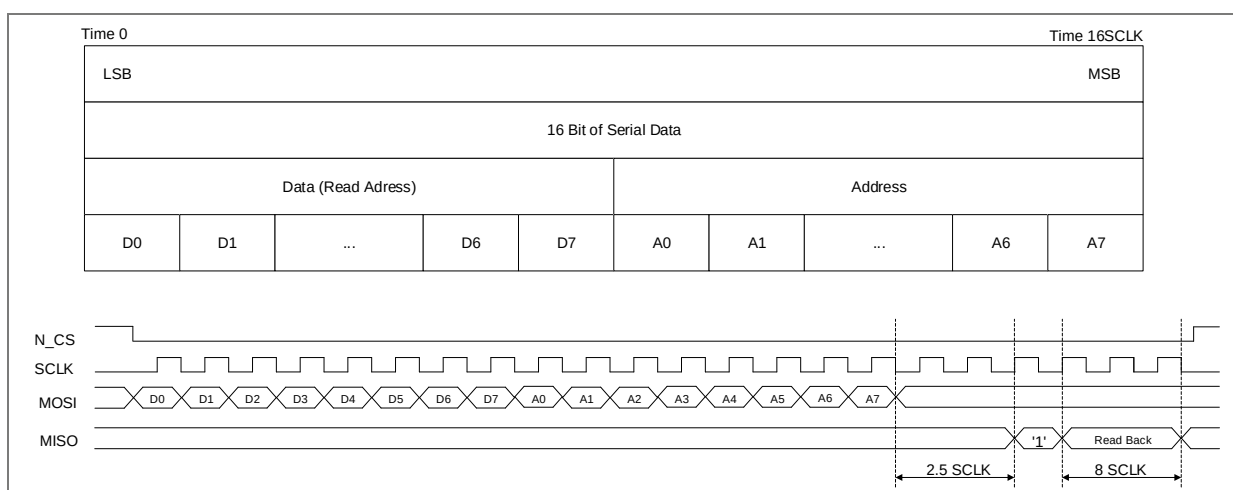
Figure 29: Reading operation
