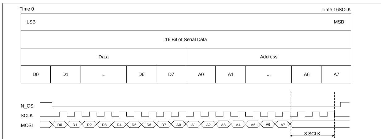
Figure 28: Writing operation
