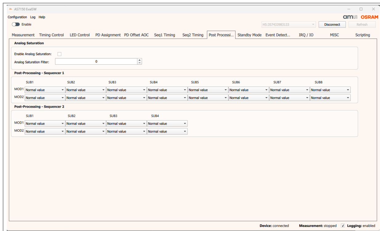
Figure 17: Post processing window
