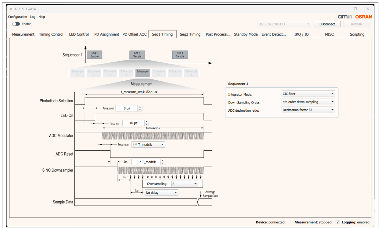
Figure 15: Sequencer 1 measurement timing window
