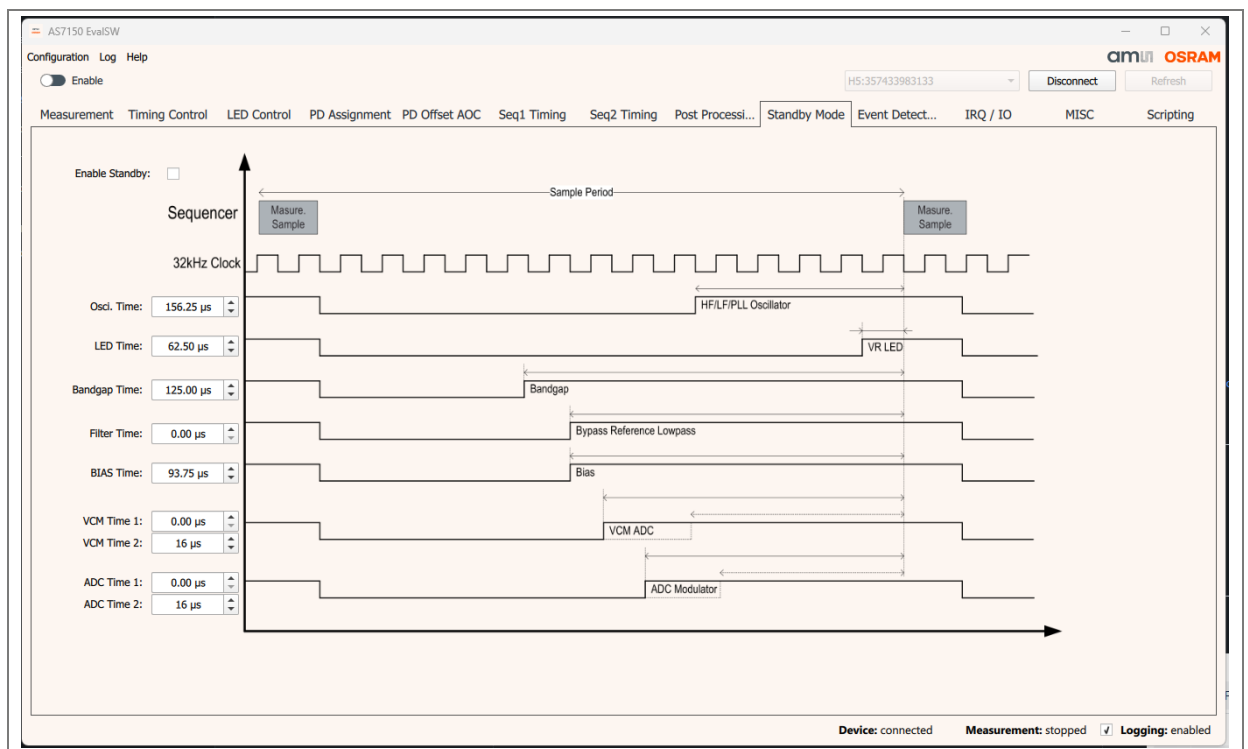
Figure 18: Standby mode window
