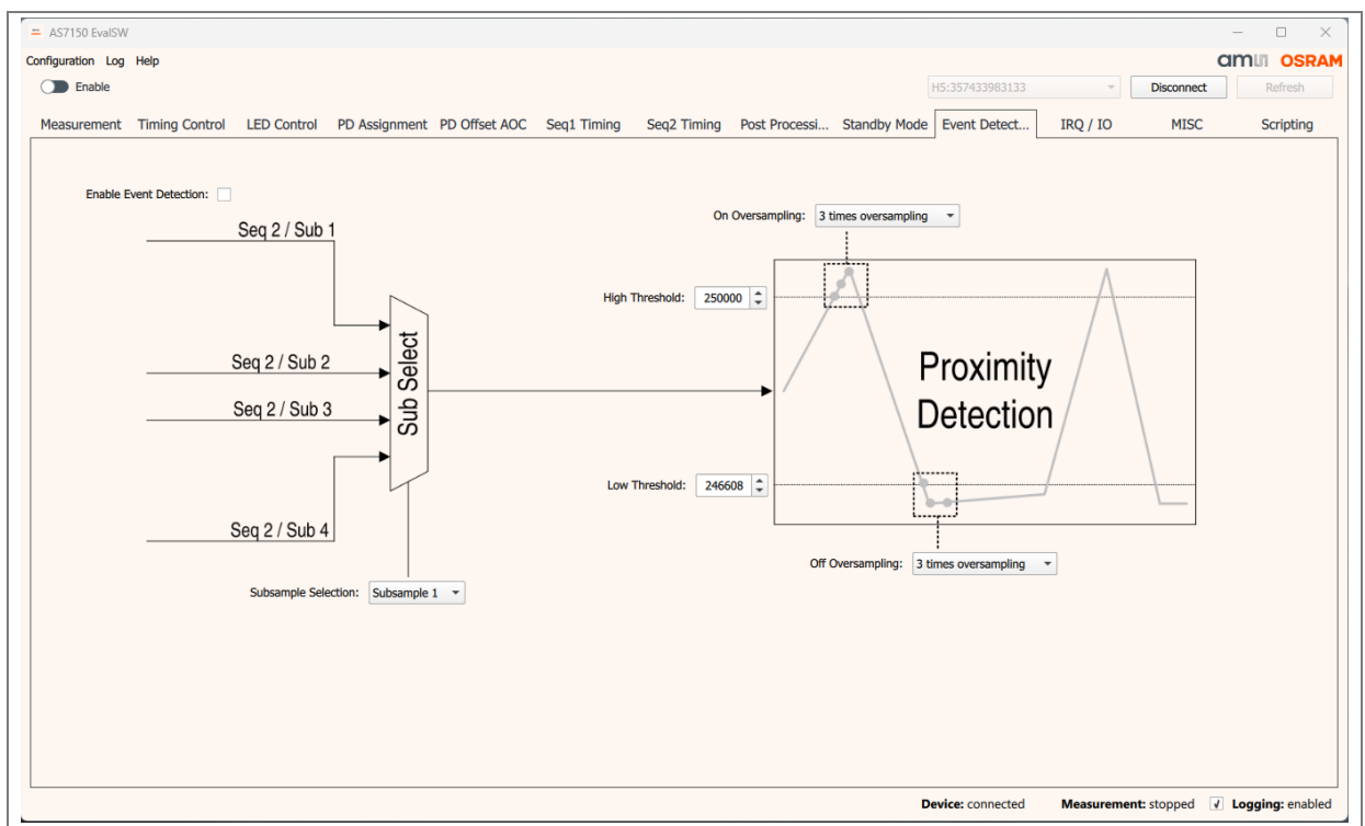
Figure 19: Event detection window
