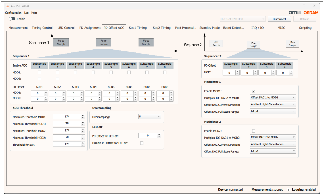
Figure 14: PD offset AOC page
