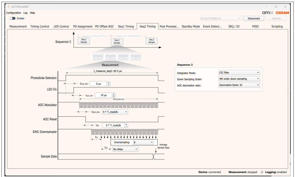
Figure 16: Sequencer 2 measurement timing window
