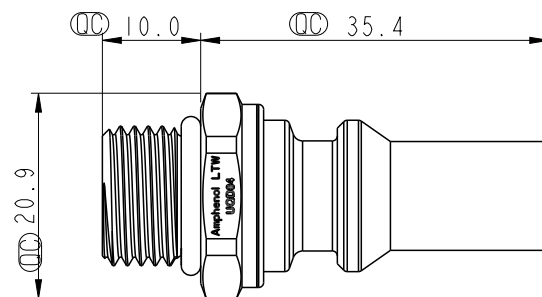
Plug
