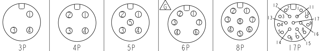
Pin Assignment Front View
