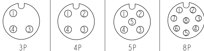
Pin Assignment Front View
