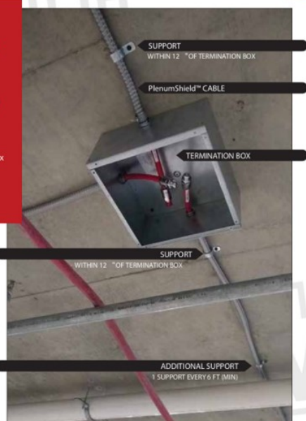
PlenumShield Typical Installation
