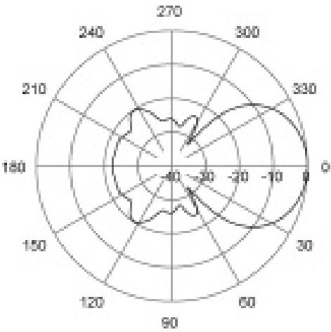
E-Plane | 340 MHz
