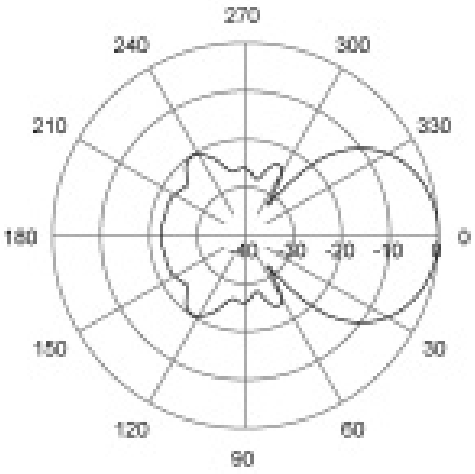
E-Plane | 330 MHz
