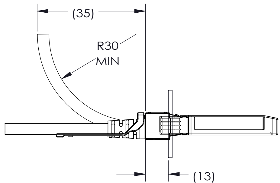
SFP+ BEND DISTANCE FROM FACEPLATE
