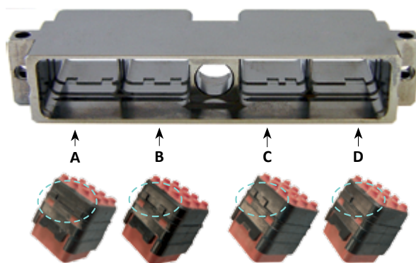
4 modules receptacle polarization
