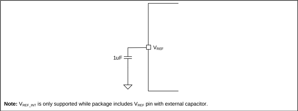
Figure 9.5-2 Typical Connection with Internal Voltage Reference
