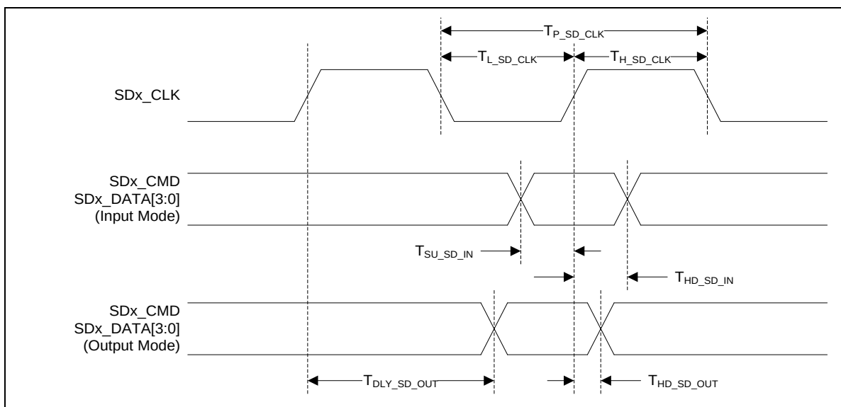
Figure 9.6-12 SDIO High-speed Mode
