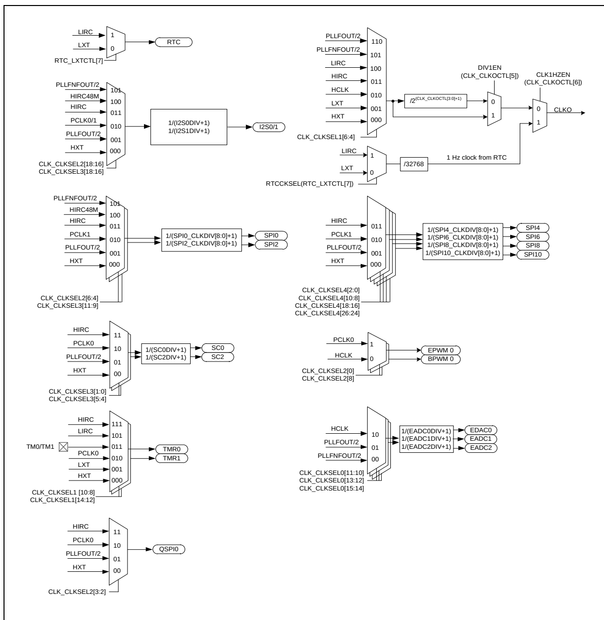
Figure 6.3-2 Clock Generator Global View Diagram (2/3)
