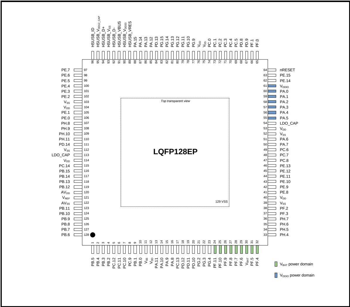
Figure 4.1-7 M463 Series LQFP128 EPAD Pin Diagram
