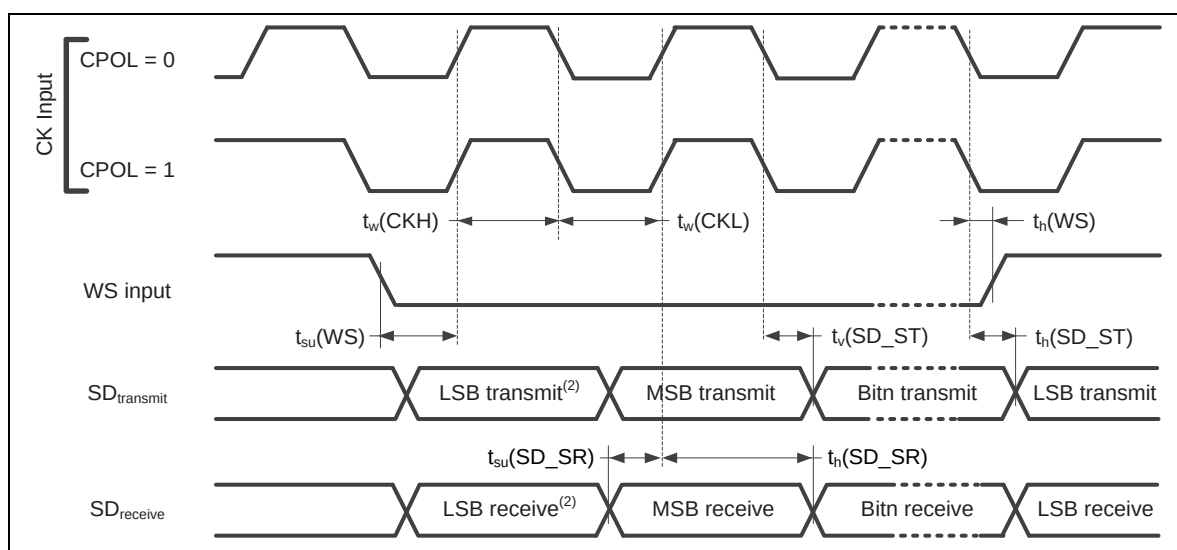
Figure 9.6-5 I²S Slave Mode Timing Diagram
