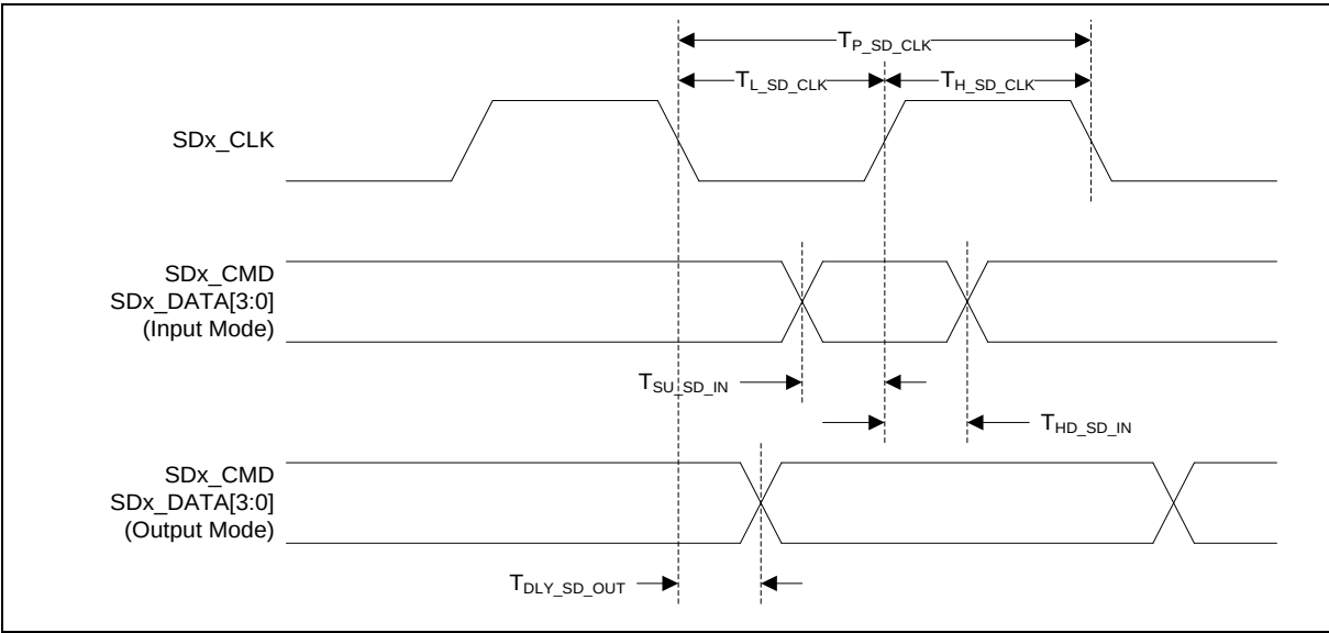
Figure 9.6-11 SDIO Default Mode
