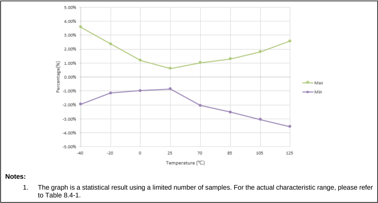
Figure 8.4-1 HIRC vs. Temperature
