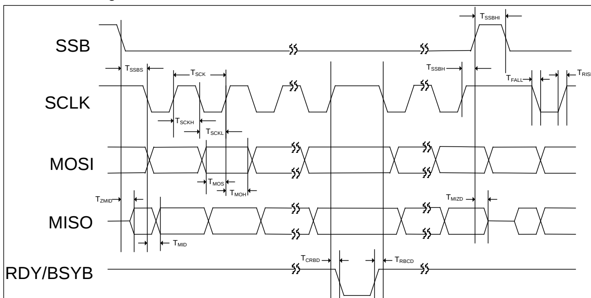
Figure 0-1 SPI Timing
