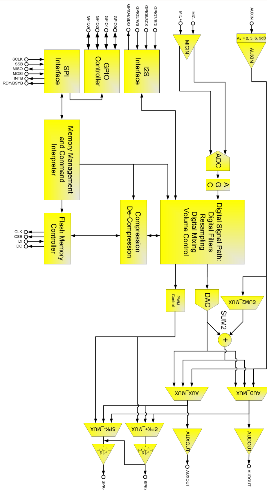
Figure 3-2 ISD15C00 Block Diagram, MICIN Selecte
