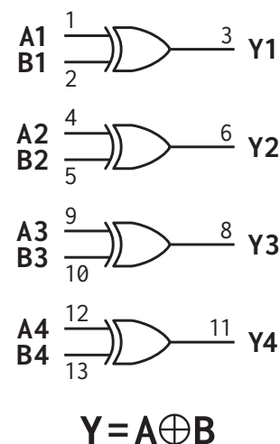
Figure 1: AP54RHC86 Logic Diagram
