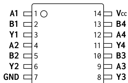
Figure 2: AP54RHC86 Device Pinout
