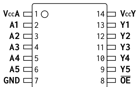
Figure 2: AF54RHC504 Device Pinout
