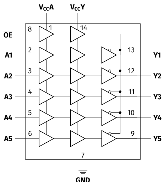
Figure 1: AF54RHC504 Logic Diagram
