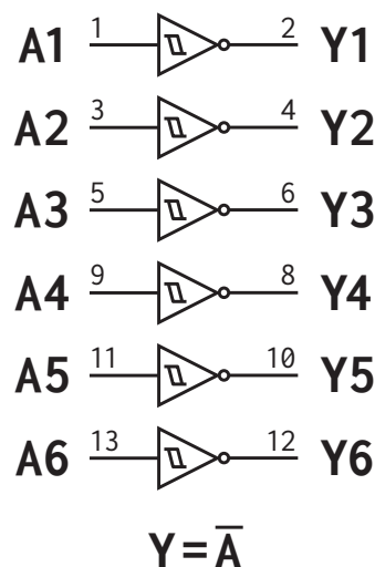
Figure 1: AF54RHC14 Logic Diagram
