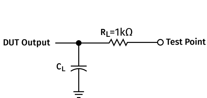
Figure 3: Load Circuit
