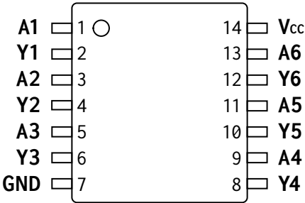
Figure 2: AF54RHC14 Device Pinout
