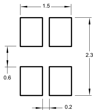
Figure 6: Recommended Soldering Land Pattern
