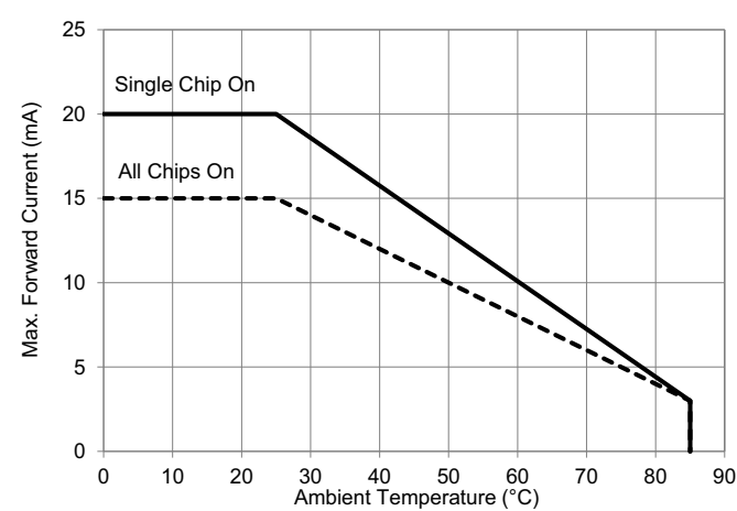
Figure 5: Derating Curve
