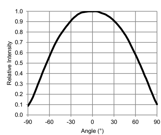
Figure 5: Relative Intensity vs. Angle
