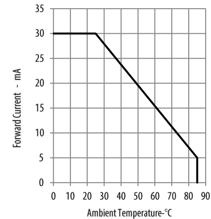
Figure 8: Derating Curve
