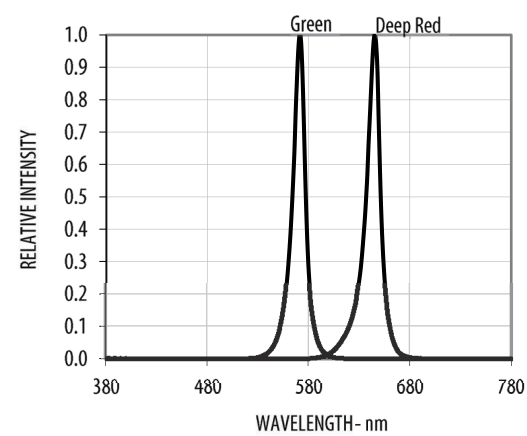
Figure 3: Spectrum
