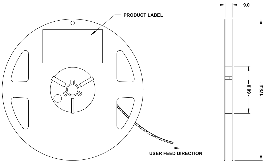
Figure 11: Reel Dimensions
