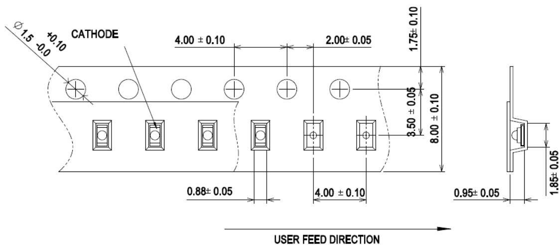
Figure 8: Carrier Tape Dimensions
