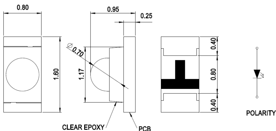
Figure 1: Package Dimensions
