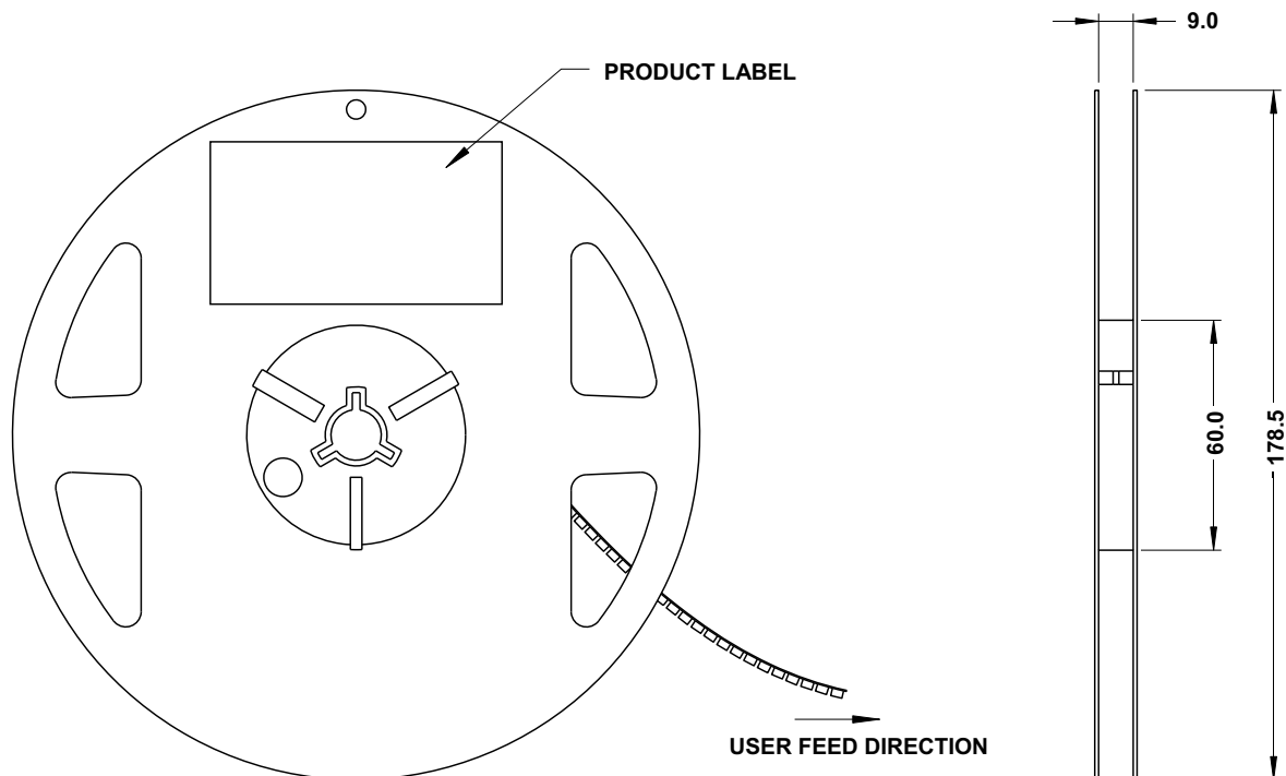
Figure 9: Reel Dimensions
