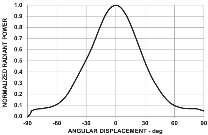
Figure 5: Radiation Pattern
