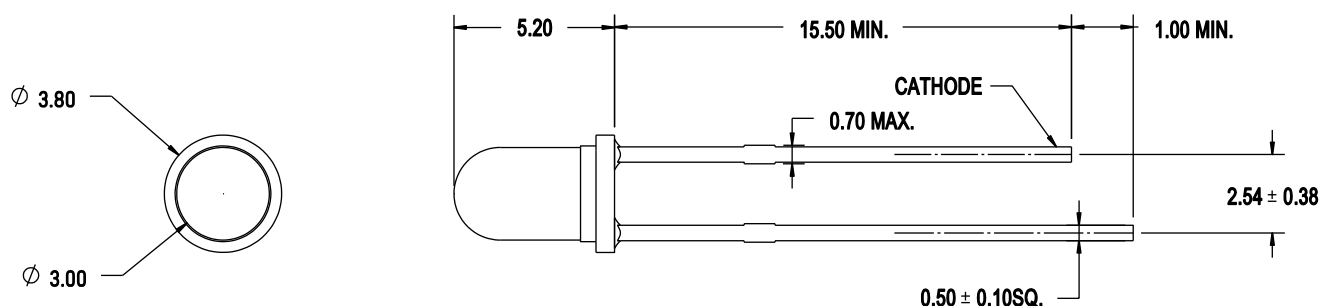
Figure 1: Package Drawing
