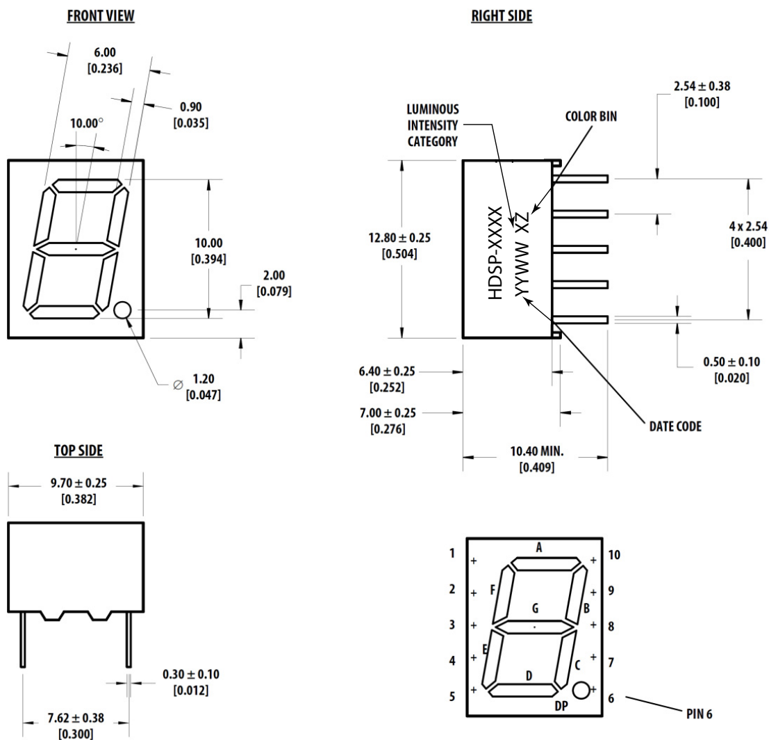
Figure 1: Package Drawing
