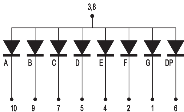
Figure 2: Internal Circuit Diagram
