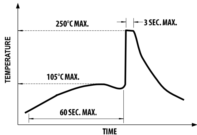
Figure 7: Recommended Wave Soldering Profile
