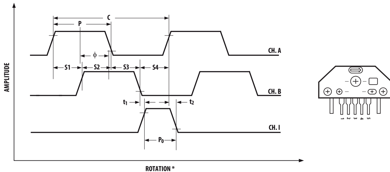
Figure 5: Output Waveforms
