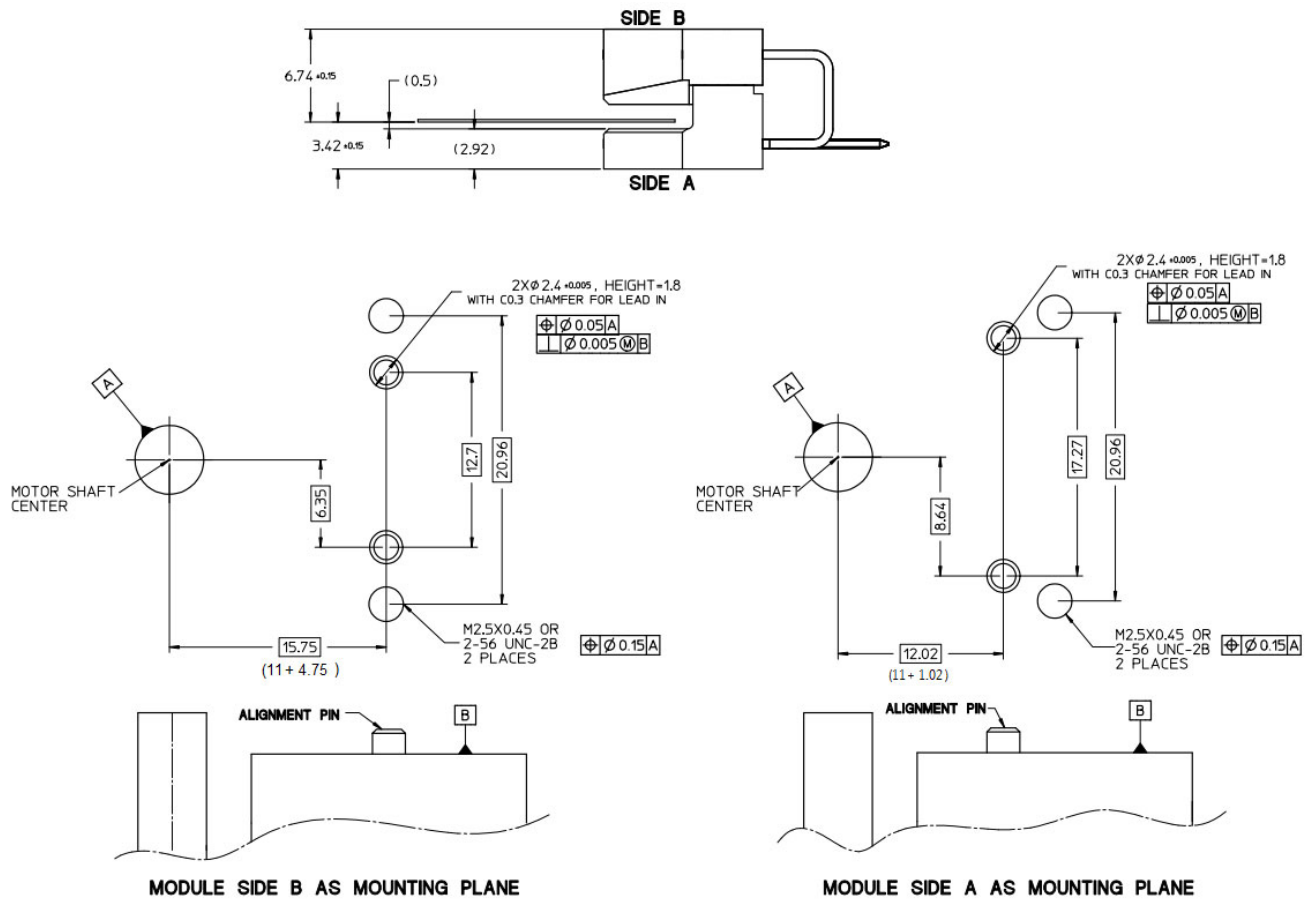
Figure 3: Mounting Considerations
