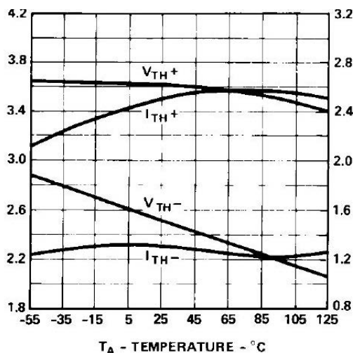
Figure 2: Typical DC Threshold Levels vs. Temperature
