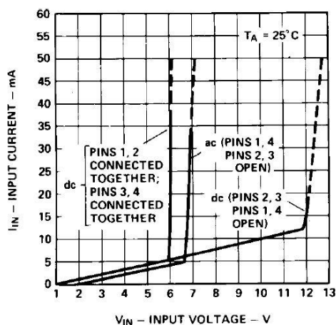
Figure 3: Typical Input Characteristics, I_{IN} vs. V_{IN} (AC Voltage Is an Instantaneous Value)
