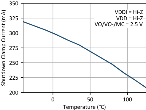
Figure 31. Shutdown Clamp Current vs. Ambient Temperature
