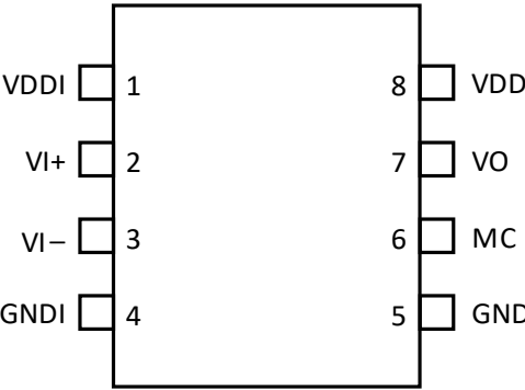
Figure 10. Si82B47x Pinout
