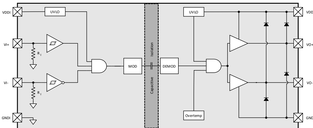
Figure 13. Si82B40x/43x with Split Output and Complementary Input
