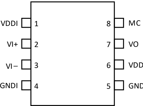
Figure 9. Si82B44x Pinout
