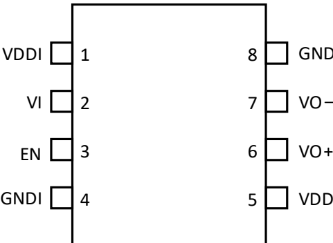
Figure 2. Si82B30x Pinout
