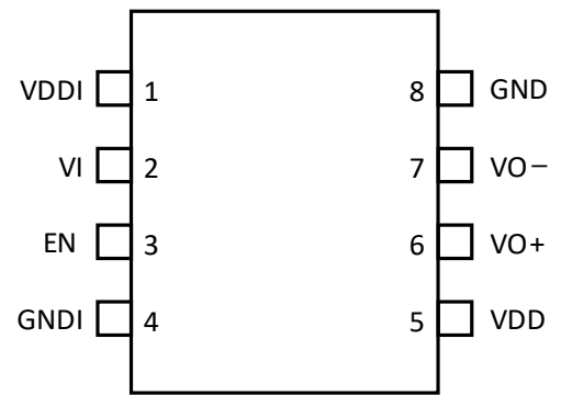
Figure 5. Si82B30x Pinout
