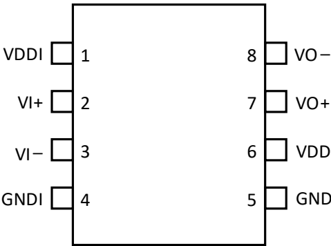
Figure 8. Si82B43x Pinout
