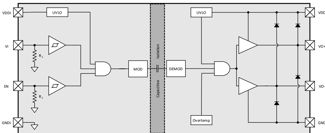
Figure 12. Si82B30x with Split Output and Enable Input
