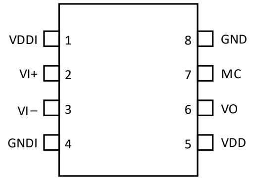
Figure 7. Si82B41x Pinout
