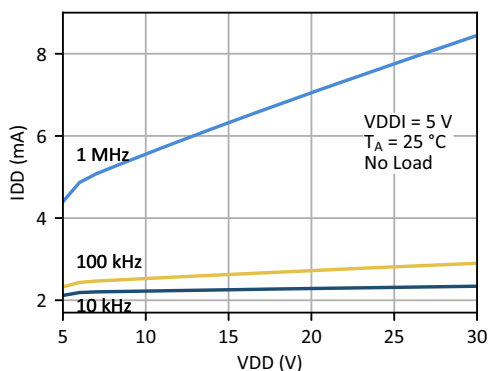
Figure 28. Gate Driver Active Supply Current vs. Gate Driver Supply Voltage
