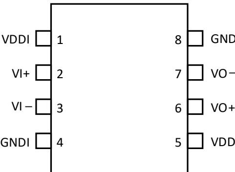
Figure 3. Si82B40x Pinout
