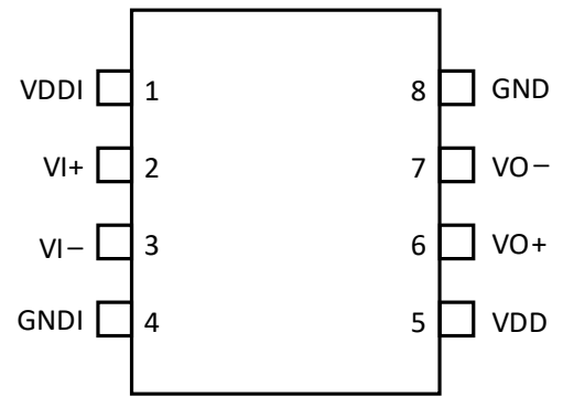
Figure 6. Si82B40x Pinout
