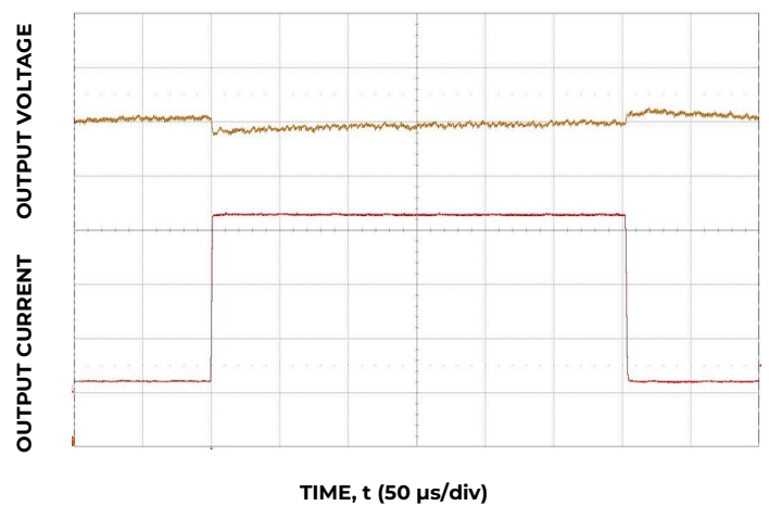
Transient response to 10 A/ \mu s Load Change from 25% to 75% at 12V IN , C_o=8x470uF+48x47uF+2x22uF+6x0.1uF
