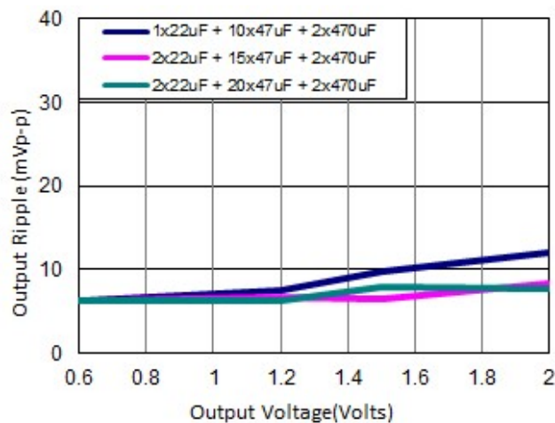
Peak to peak output ripple voltage for various output voltages with external capacitors at the output (30 A load). Input voltage is 12V.
