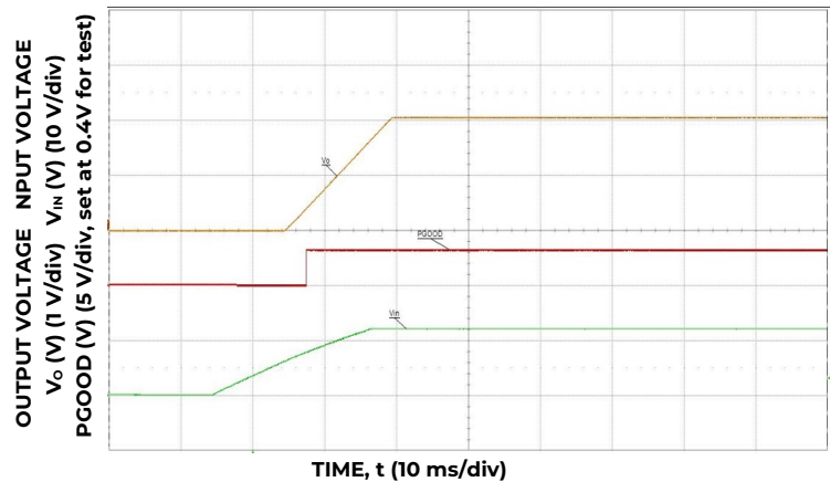
Typical Start-up Using Input Voltage ( V_{IN} = 12V , V_{OUT} = 1.8V , I_o = I_{o,max} ).
