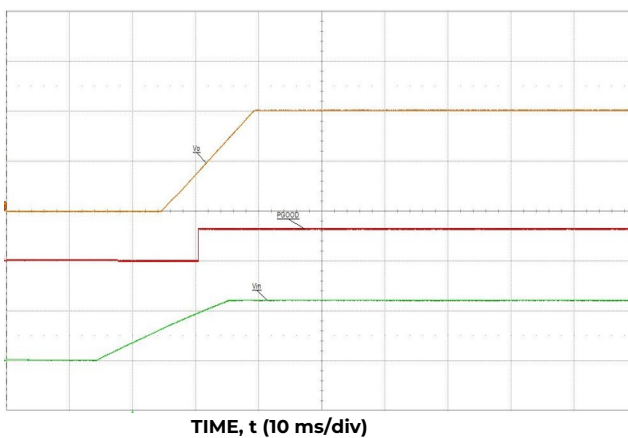
Typical Start-up Using Input Voltage (V IN =12V, I o =I o,max ).
