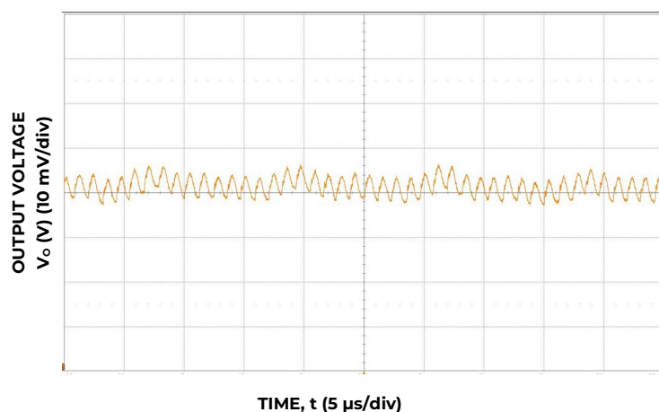
Typical output ripple, C O =8x470uF+48x47uF+2x22uF+6x0.1uF, V IN =12V, I o =I o,max
