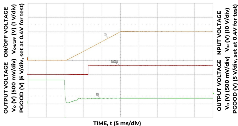
Typical Start-up Using On/Off Voltage (I o =I o,max ).
