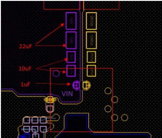
1 \mu\text{F} & 10 \mu\text{F} Capacitor under V_{\text{IN}} Pad
