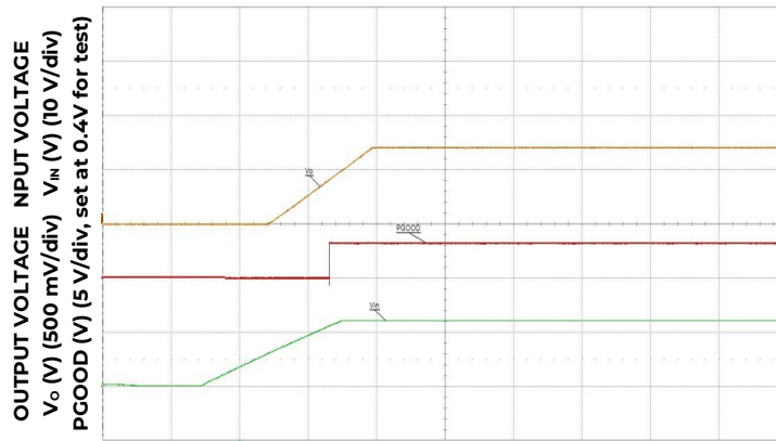
TIME, t (10 ms/div)
