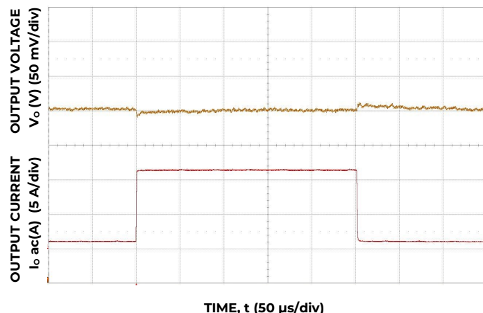
Transient response to 10 A/ \mu s Load Change from 25% to 75% at 12VIN, C_o=8x470uF+48x47uF+2x22uF+6x0.1uF
