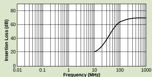
Insertion Loss 1212-0502
